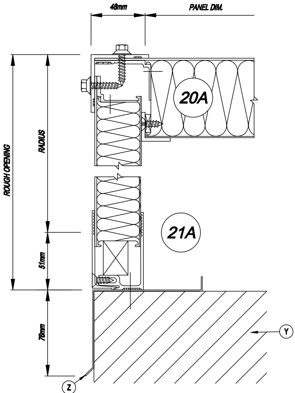
TYPICAL JAMB DETAIL.
